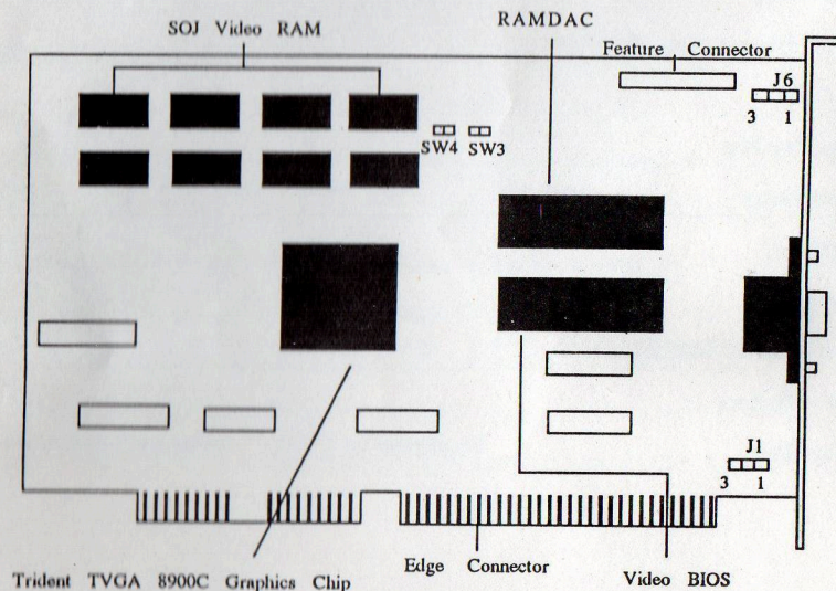
Figure-1B TVGA 8900C SOJ graphics layout
