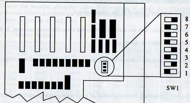
Figure-6 With a ballpoint pen set SW1, positions 5 and 6, to ON
