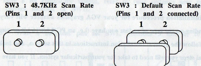
Figure-4 SW3 Setting For Selecting Scan Rate
